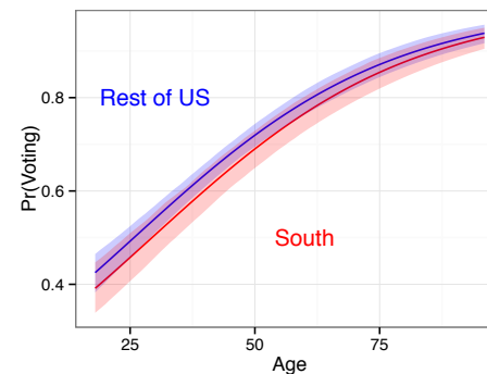
Predicted probabilities - simulated data (ggplot2)
