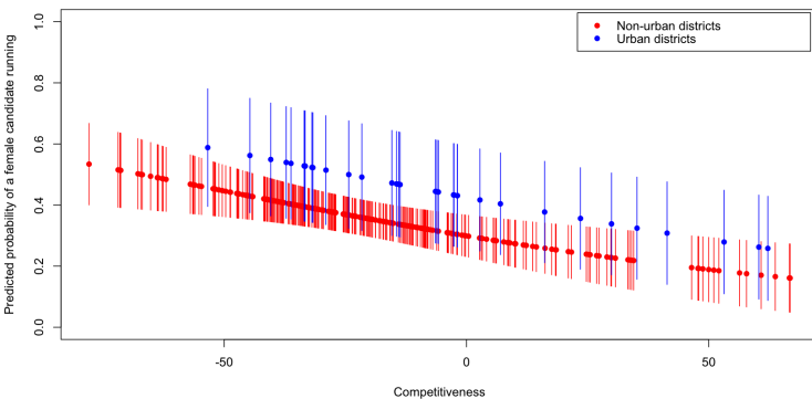
Predicted probabilities - simulated data (base plot)
