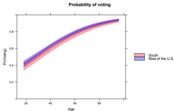
Predicted probabilities - simulated data (lattice plot)
