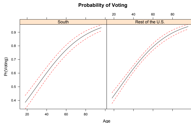
Predicted probabilities - simulated data (lattice plot)
